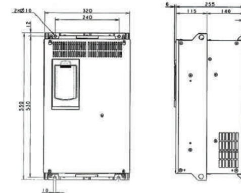
External dimensions (mm) 30 kW
