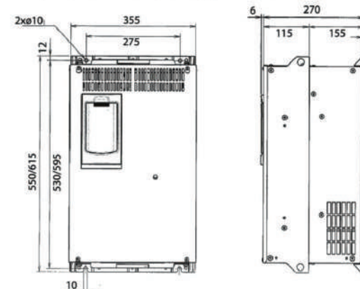
External dimensions (mm) 37 and 45 kW
