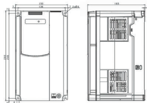
External dimensions (mm) 4.0 kW
