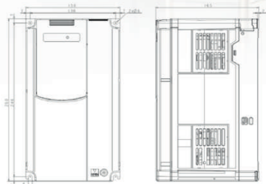
External Dimensions (mm)
