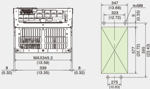
Panel cutout dimensions for external cooling
