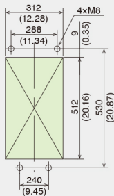
Panel cutout dimensions for external cooling
